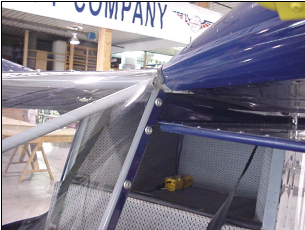
The top screw also picks up on Door Sill 7F19-12D
