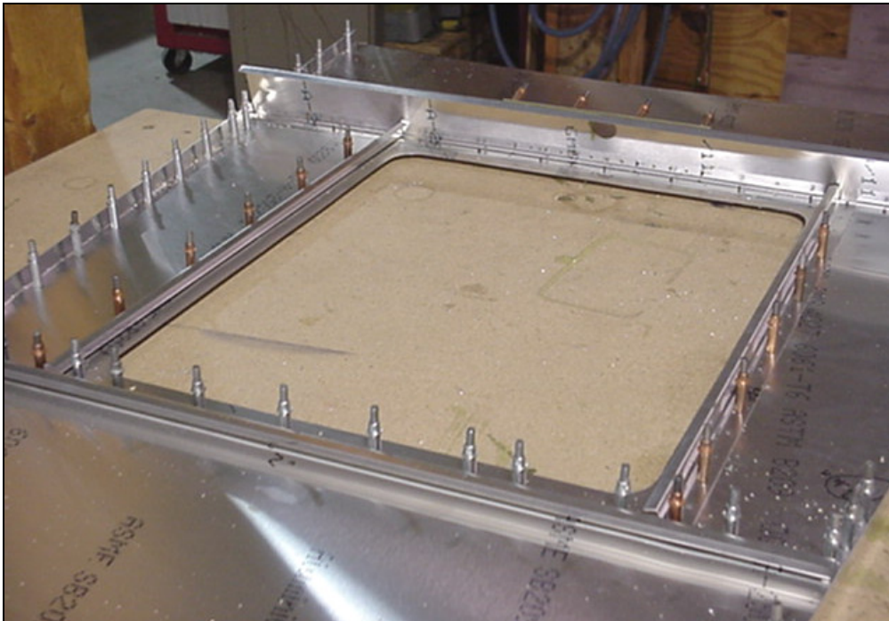
View of the two 'Z' in the Bottom Skin.
