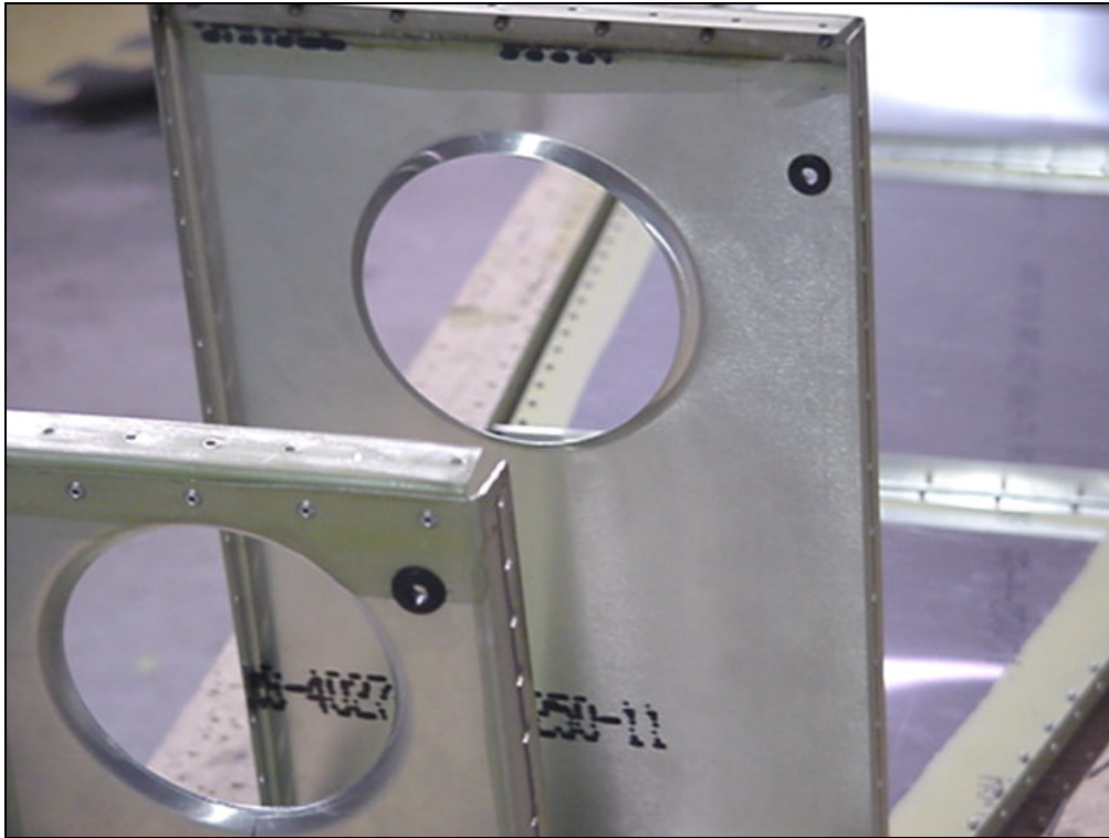
7F1-3 Rear Horizontal Tail Frame 7F1-4 Front Horizontal Tail Frame
