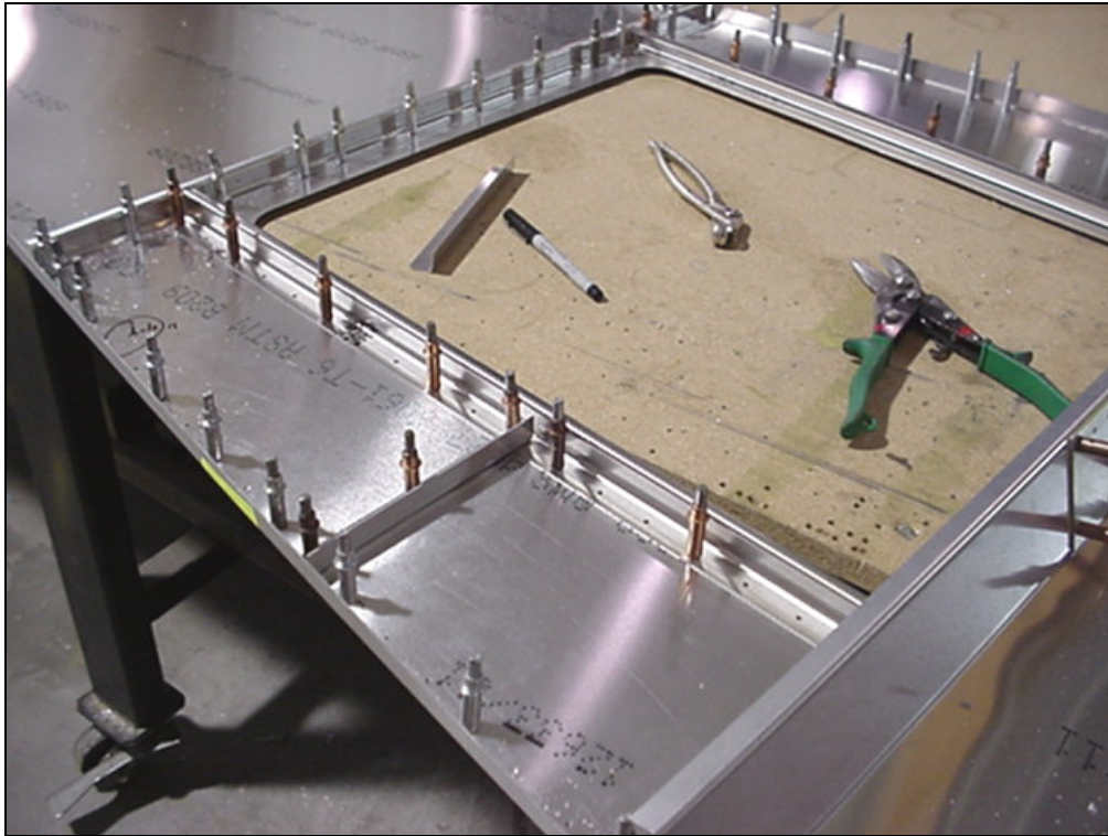
Short L angles Ref. 7-F-6
