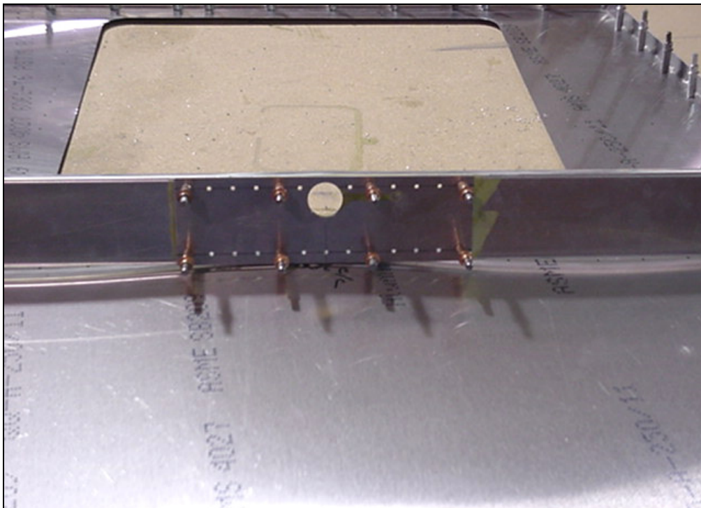
7F6-1 Bottom Channel 7F2-3 Bottom Skin
