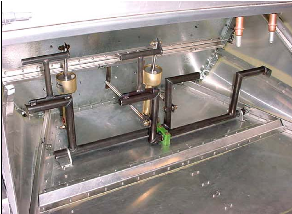
Dual Rudder Pedals with toe brakes on pilot side
