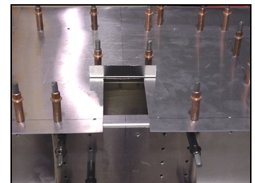
L Angle along front of cutout.
