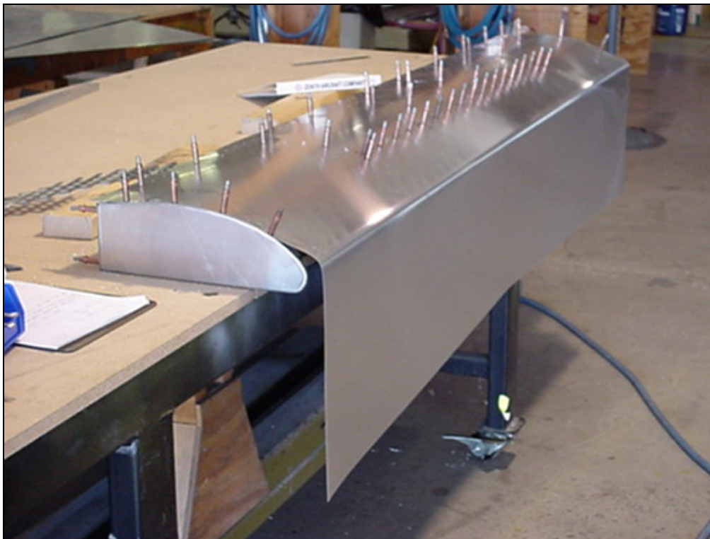
Photo of bottom side of stabilizer
