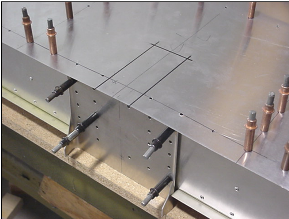
Cutout on top side only of stabilizer skin (to make room for the upper elevator cable)
