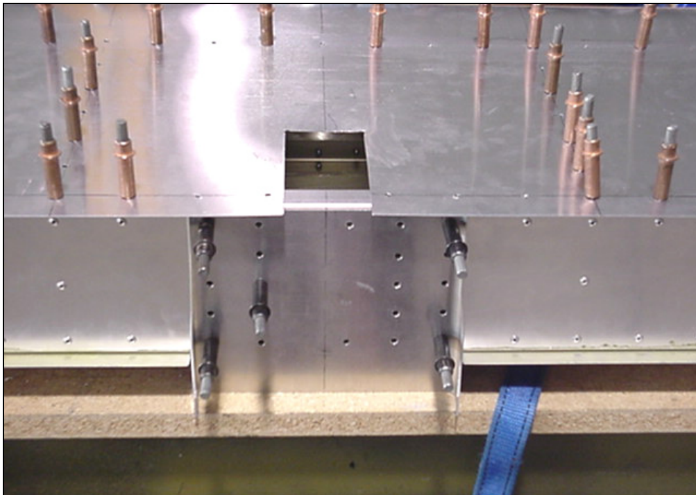
Elevator cutout on top of Stabilizer
