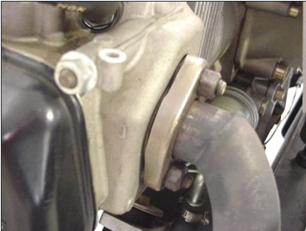
Do not over torque the muffler bolts, notice the gap at the top and bottom of the exhaust socket and the engine.
