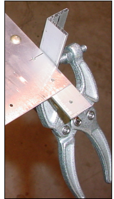
Clamp a piece of extrusion or other piece of flat plate to the bottom flange of the spar (centered on the rib rivet line).
