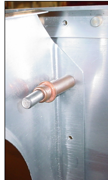
Detail of rear rib spar flange overlapping on the main wing spar 7W2-1
