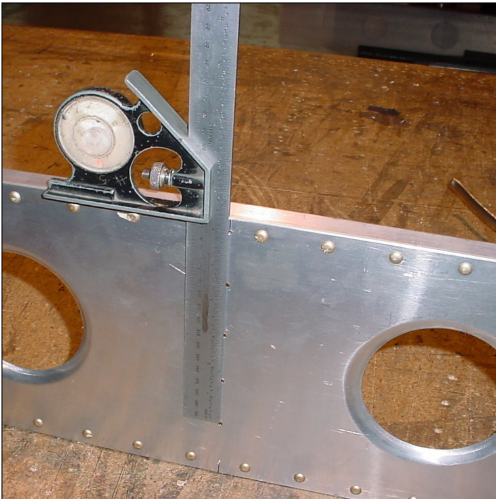
Assembly of the right wing skeleton.
