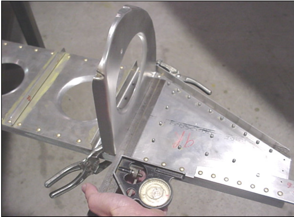
Mark rivet line on the back side of the spar flange of each nose rib. RIB ORIENTATION: All ribs are positioned with the flanges pointing towards the outboard wing tip.
