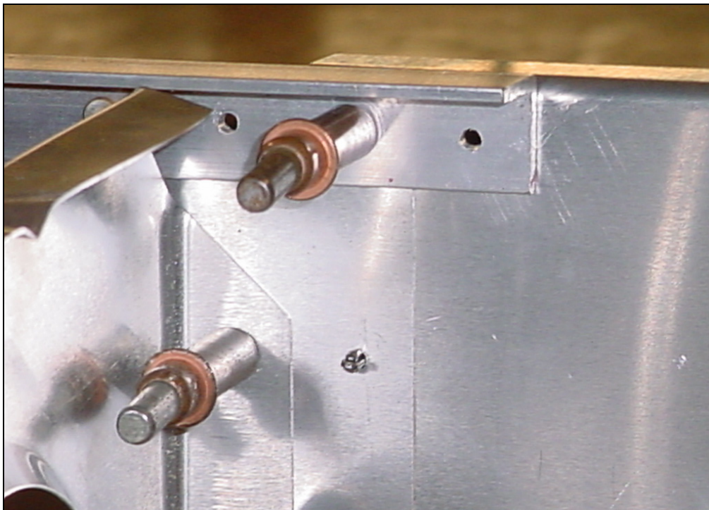
Rear view of the spar.
