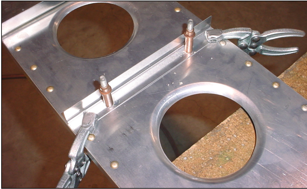
Drill and cleco with #30 drill.
