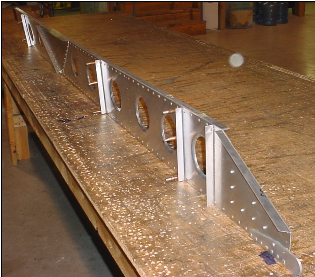
Drill and cleco with #30 drill.
