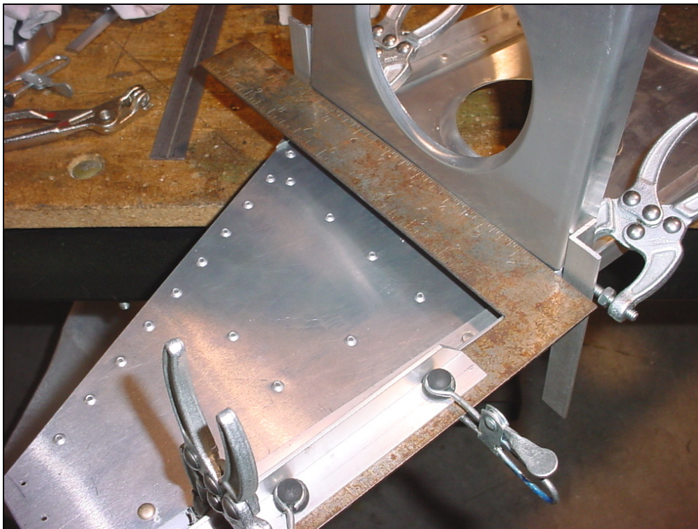
7-V-2 Rear ribs (3 flanged lightening holes).
