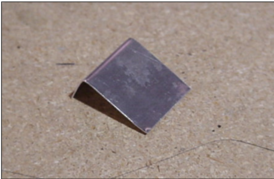
Rear Rib Angle from 7V6-3 Length = 40mm long.
