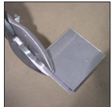
Cut in from both flanges, then twist off.
