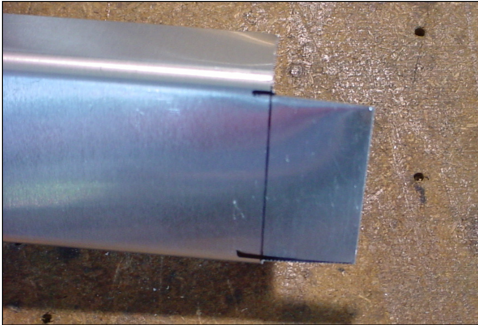
File corner relief hole with 1/4" round file.
