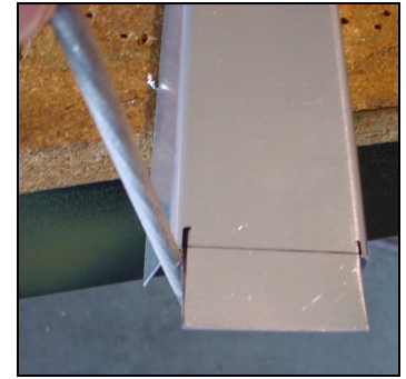
File corner relief hole with 1/4" round file.
