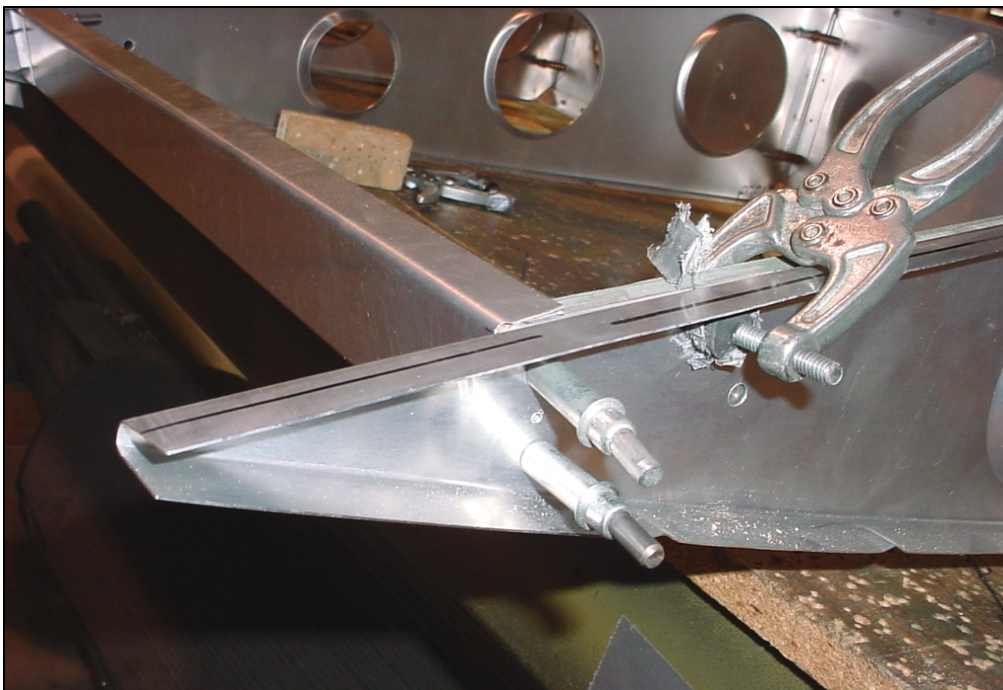
Detail: view from inboard side.
