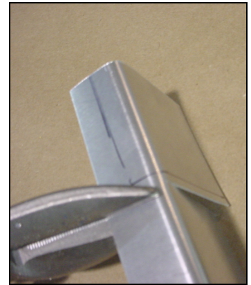
Cut in from both flanges, then twist off.
