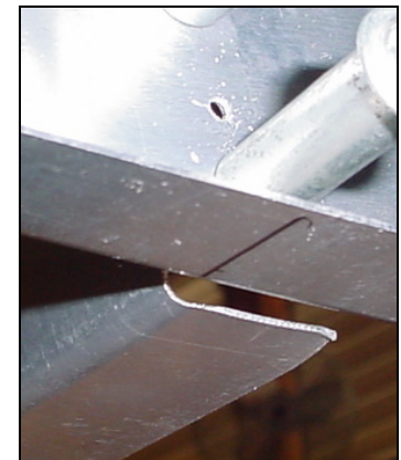
Detail, aft edge of the channel on the bottom flange of the rear rib.
