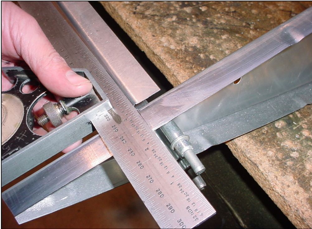
Detail: aft edge of the channel on the top flange of the rear rib.
