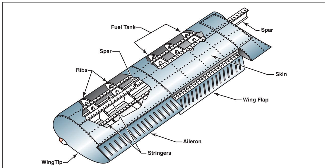
Figure 1-6. Wing components.
