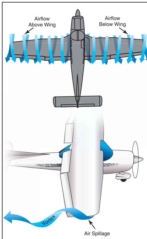
Figure 3-4. Wingtip vortices.
