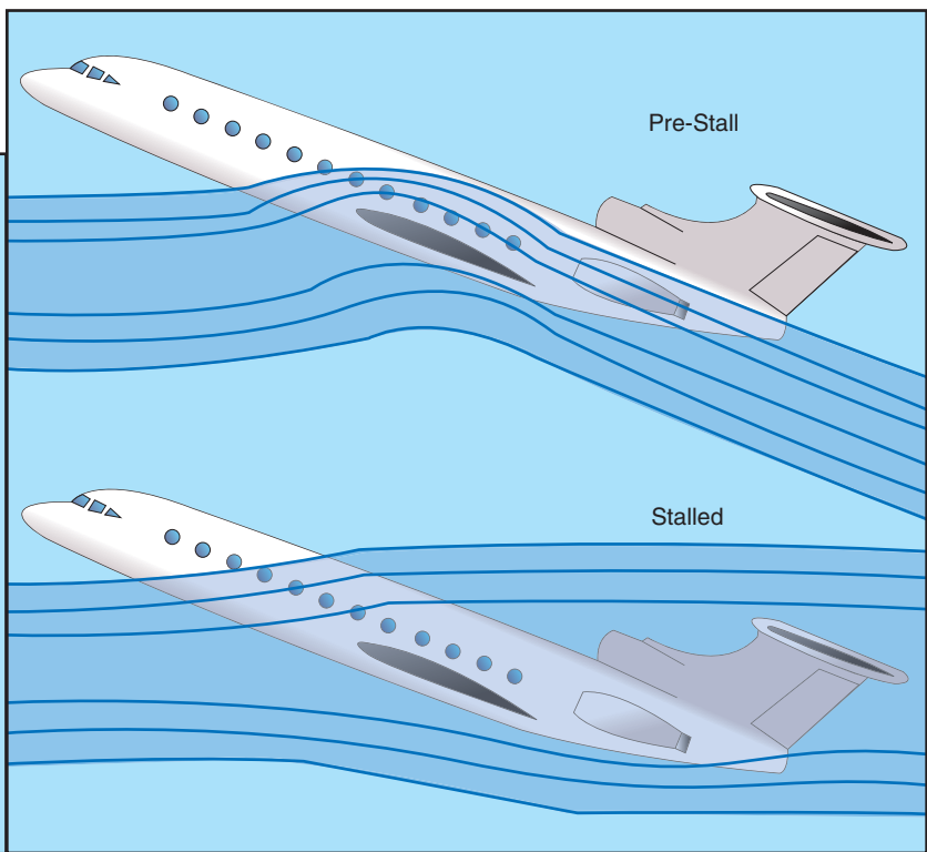
Figure 3-46. T-tail stall.
