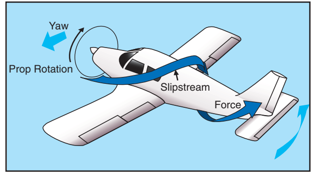
Figure 3-31. Corkscrewing slipstream.
