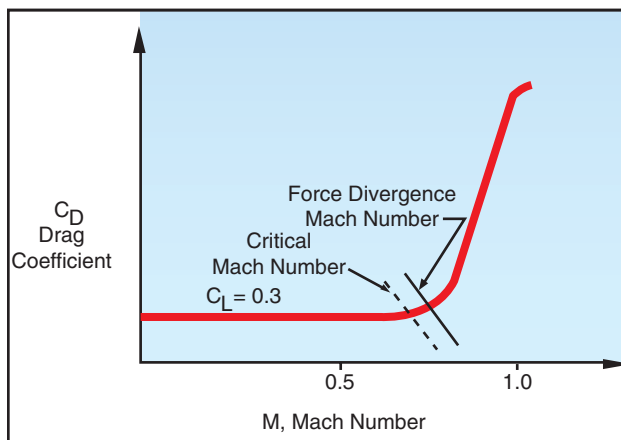
Figure 3-41. Critical Mach.
