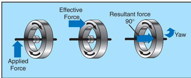
Figure 3-32. Gyroscopic precession.
