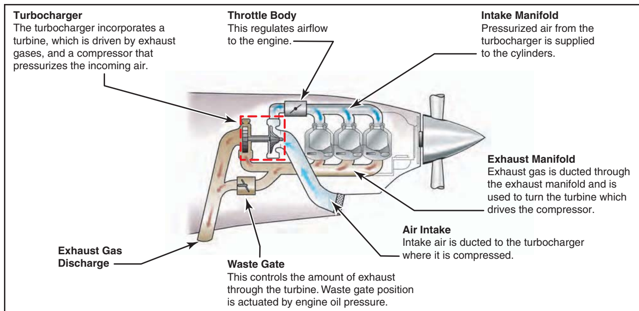
Figure 5-12. Turbocharger components.
