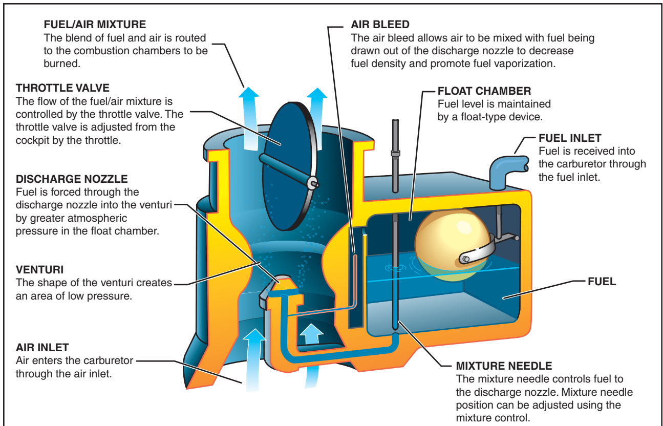
Figure 5-7. Float-type carburetor.
