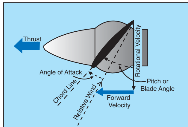
Figure 3-27. Propeller blade angle.
