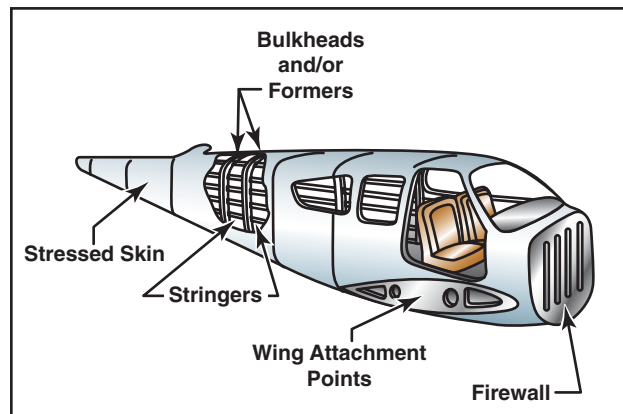
Figure 1-4. Semi-monocoque construction.
