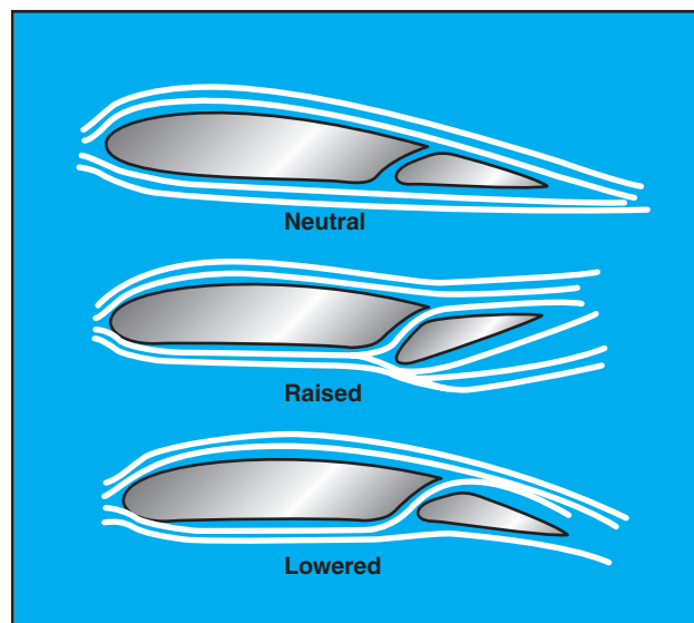
Figure 4-4. Frise-type ailerons.
