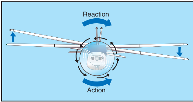
Figure 3-30. Torque reaction.
