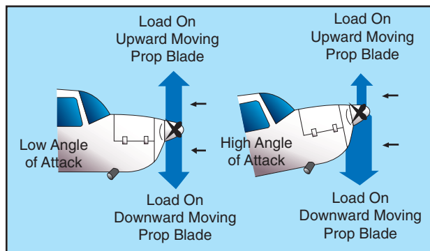
Figure 3-34. Asymmetrical loading of propeller (P-factor).
