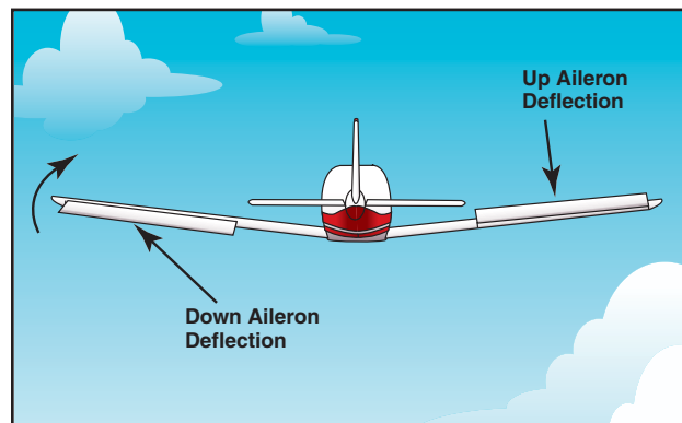
Figure 4-3. Differential ailerons.
