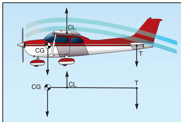
Figure 3-12. Longitudinal stability.
