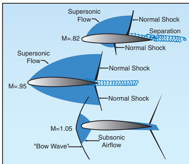
Figure 3-43. Shock waves.
