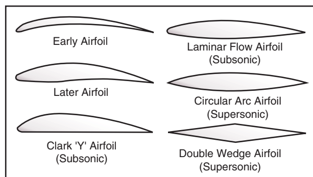
Figure 2-6. Airfoil designs.
