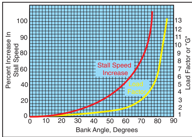
Figure 3-25. Increase in stall speed and load factor.
