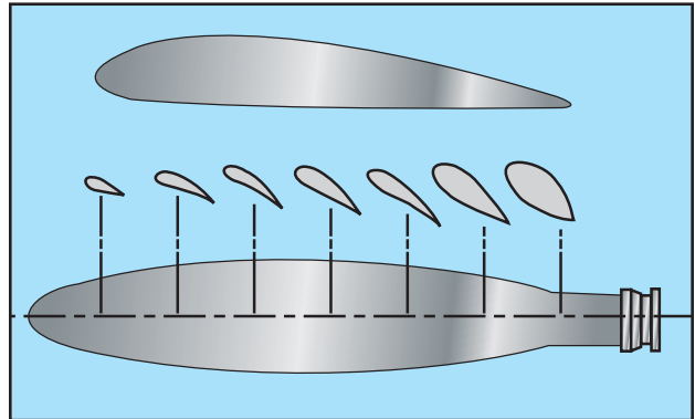
Figure 3-26. Airfoil sections of propeller blade.
