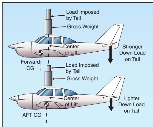
Figure 3-39. Load distribution affects balance.
