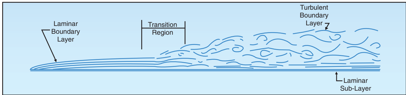
Figure 3-42. Boundary layer.
