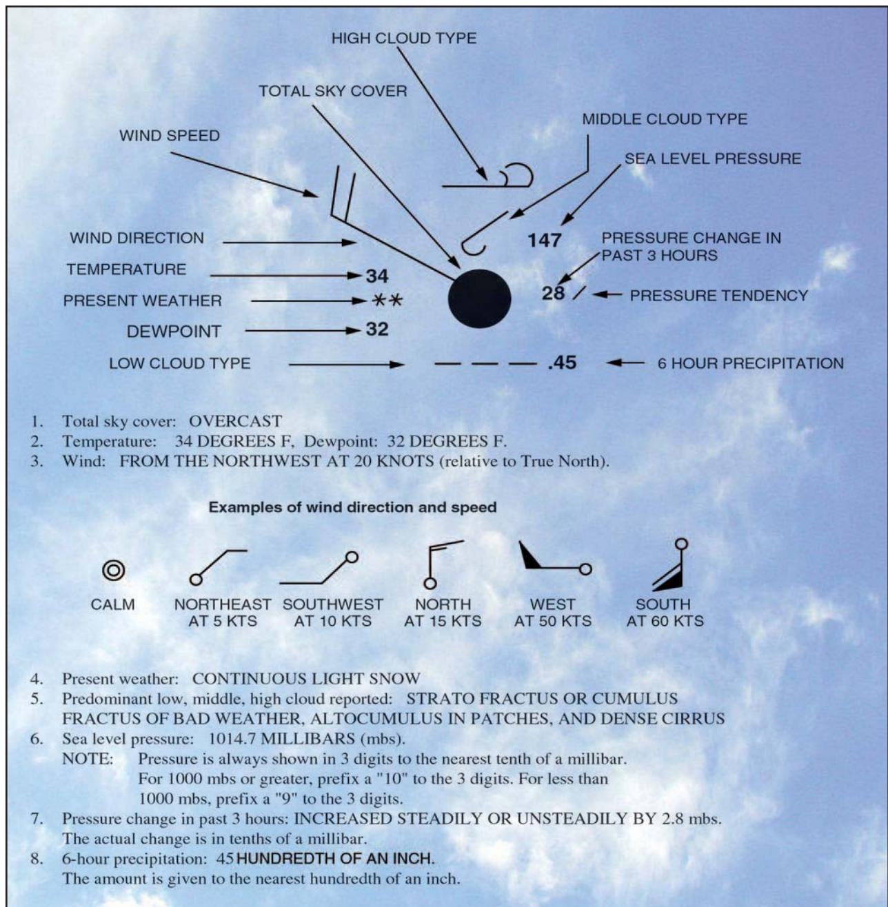
Figure 11-9. Sample station model and weather chart symbols.
