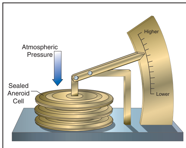
Figure 10-5. Aneroid barometer.
