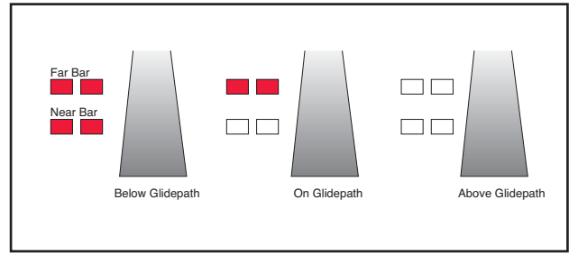
Figure 12-6. 2-Bar VASI system.
