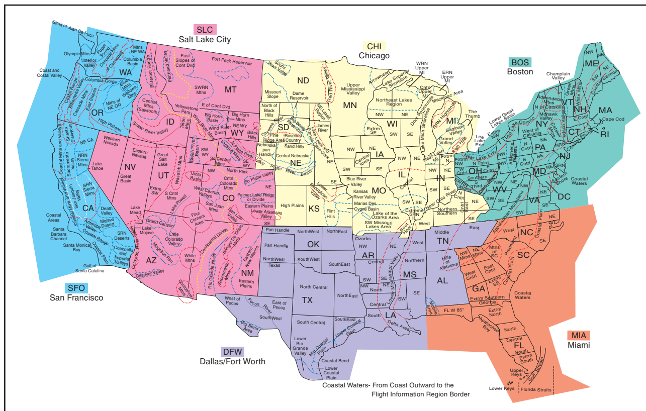
Figure 11-6. Area forecast region map.
