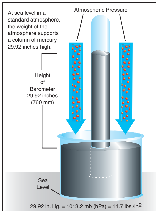
Figure 10-4. Mercurial barometer.
