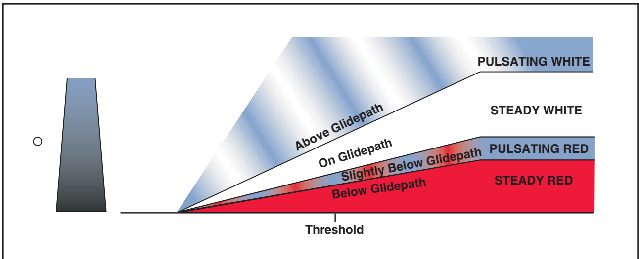
Figure 12-9. Pulsating visual approach slope indicator.
