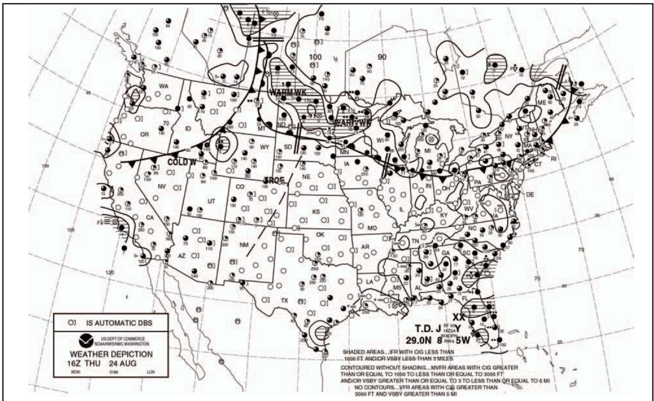
Figure 11-10. Weather depiction chart.
