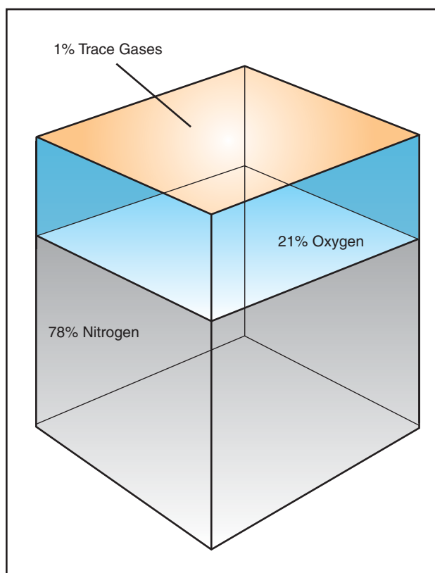
Figure 10-1. Composition of the atmosphere.
