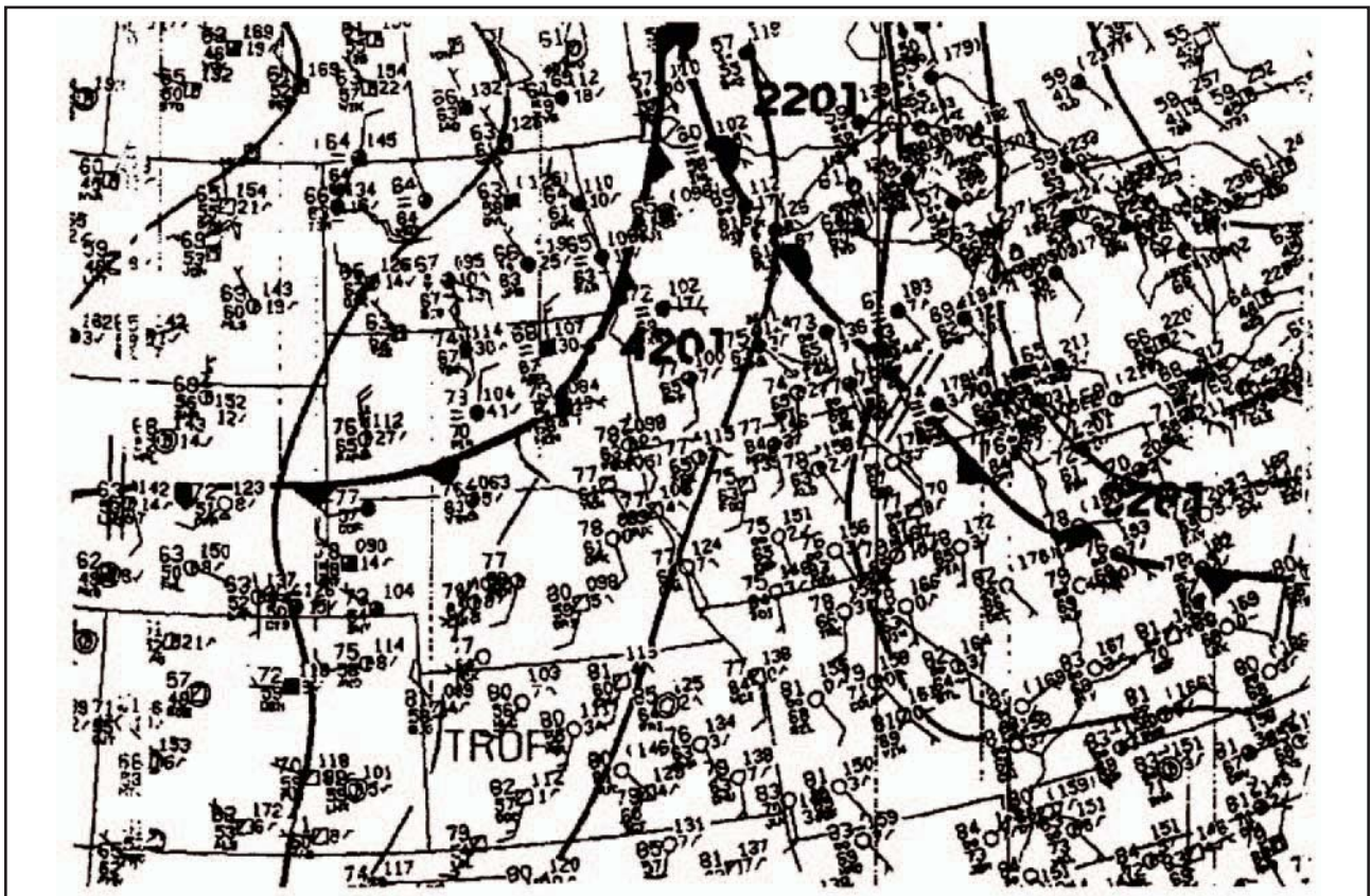
Figure 11-8. Surface analysis chart.
